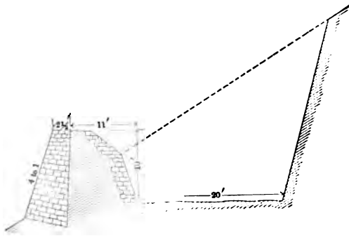
FIG. 66.—Rock Cross-section, Turlock Canal.
